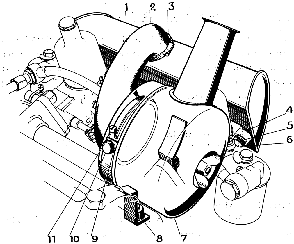
Air cleaner with induction silencer fitted on P 544
