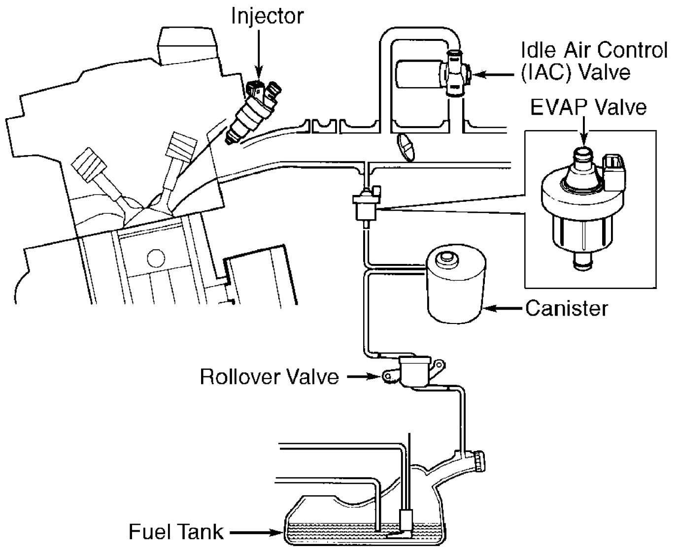
Fig. 2: Identifying EVAP System Components Courtesy of Volvo Cars of North America.
