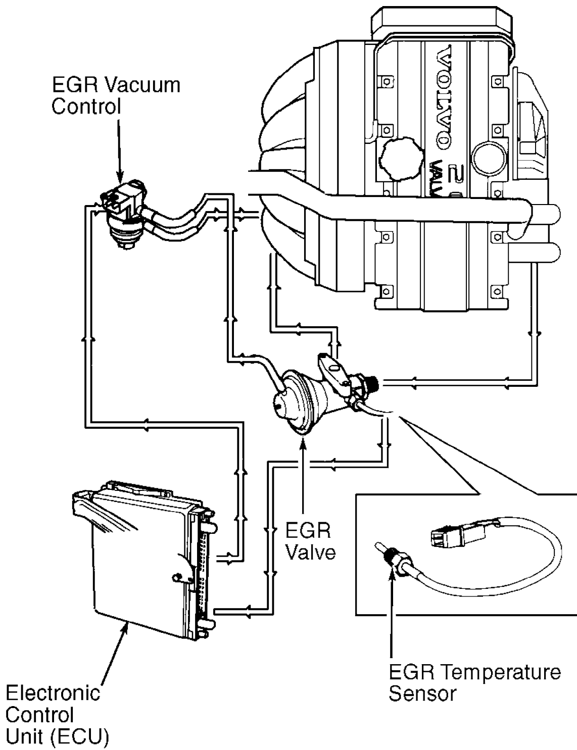
Fig. 3: Identifying EGR System Components Courtesy of Volvo Cars of North America.
