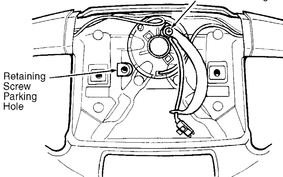
Fig. 2: Removing Steering Wheel Courtesy of Volvo Cars of North America
