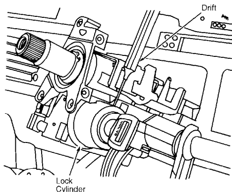
Fig. 6: Removing Ignition Switch Connector Courtesy of Volvo Cars of North America.
