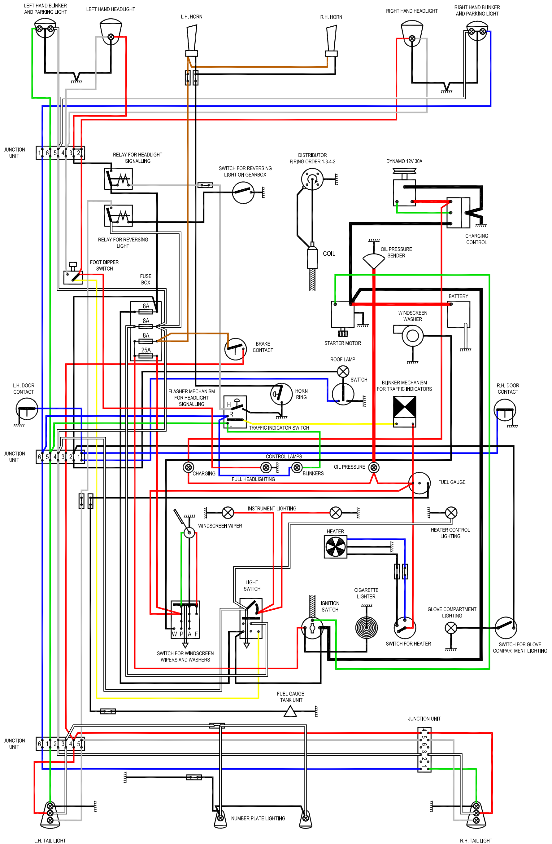
Wiring diagram. Chassis 8275 to 17949 Station Wagon
