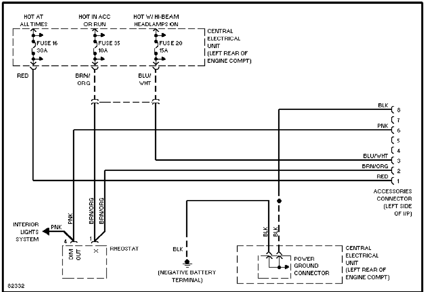
Accessories Connector Circuit, Late Production
